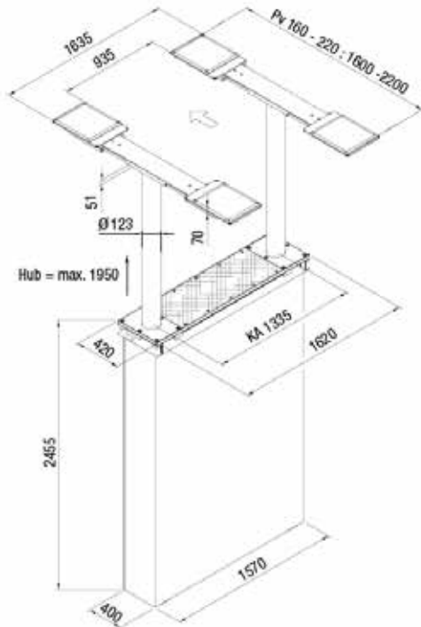
Olio idraulico 17 l. Oil filling 17 ltr.
